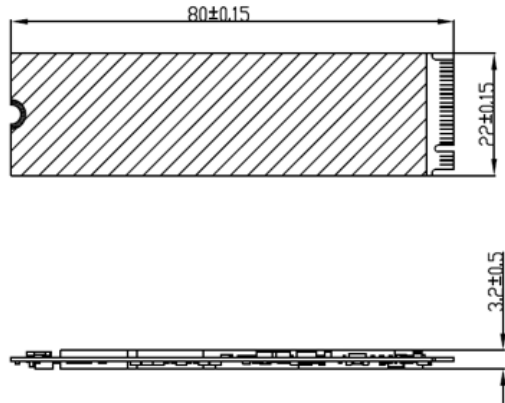
<Without heatsink>
