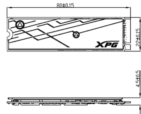
<With heatsink>
