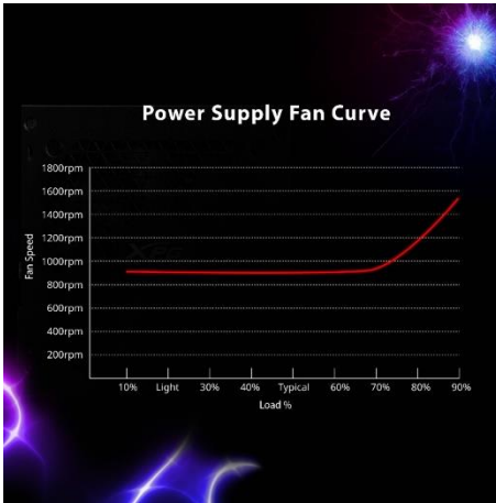
Intelligent Fan-Curve Design
